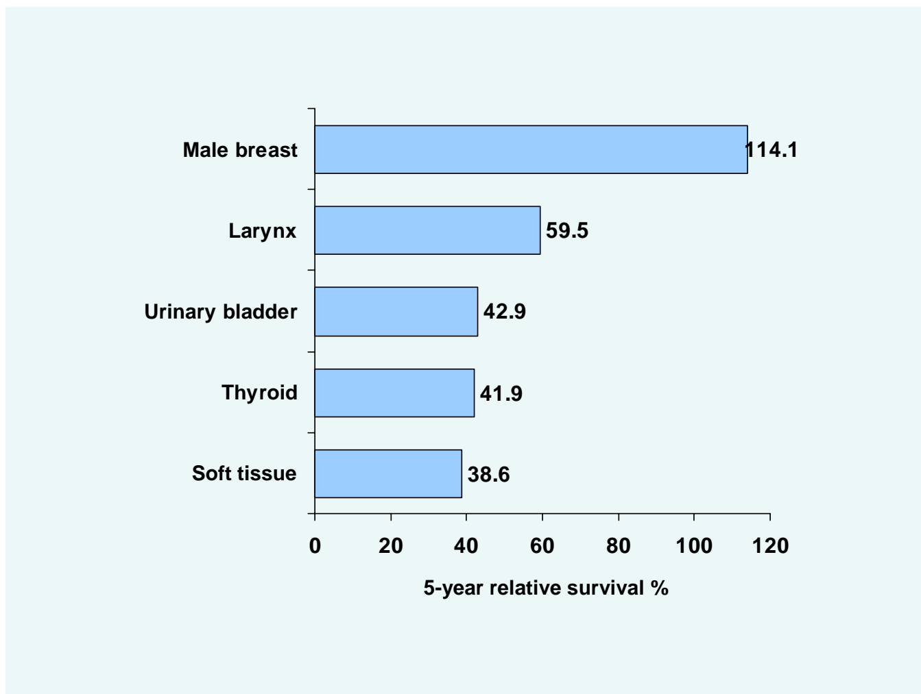
Figure 1b. Top five cancers (ranked on survival), Male, Qidong, China, 1992–2000
